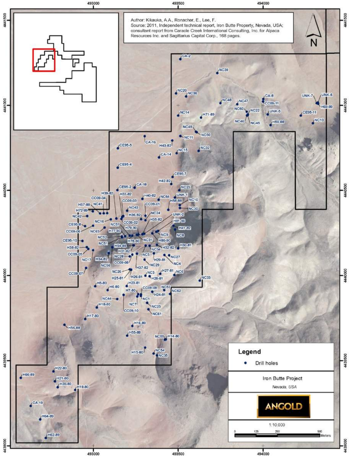
Figure 3. Location of reverse circulation drill holes drilled by previous companies (1980-2009).
