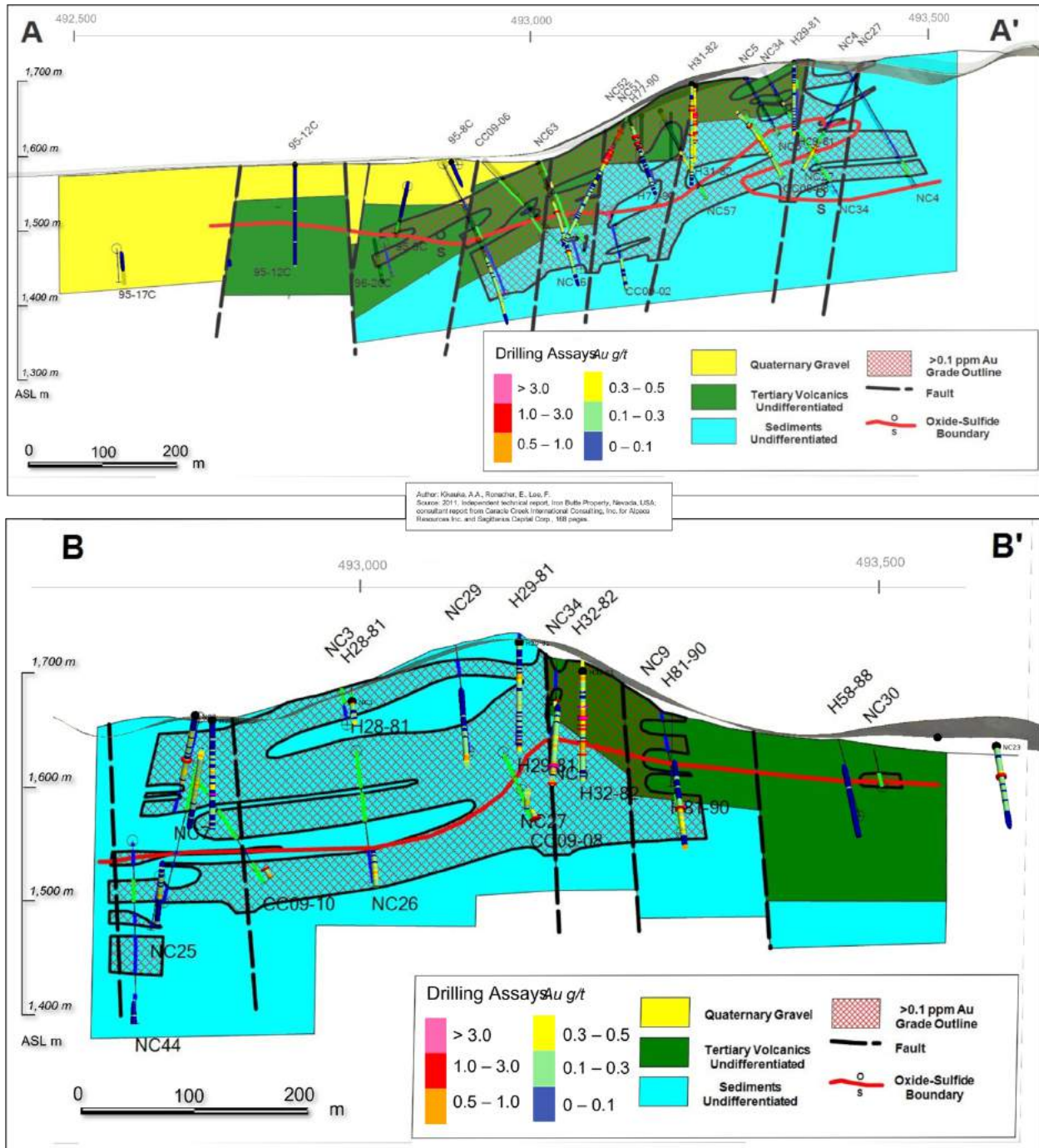
Figure 10. Cross-sections A-A' and B-B' (see Figure 9) showing outlines of 0.1 g/t Au values.
