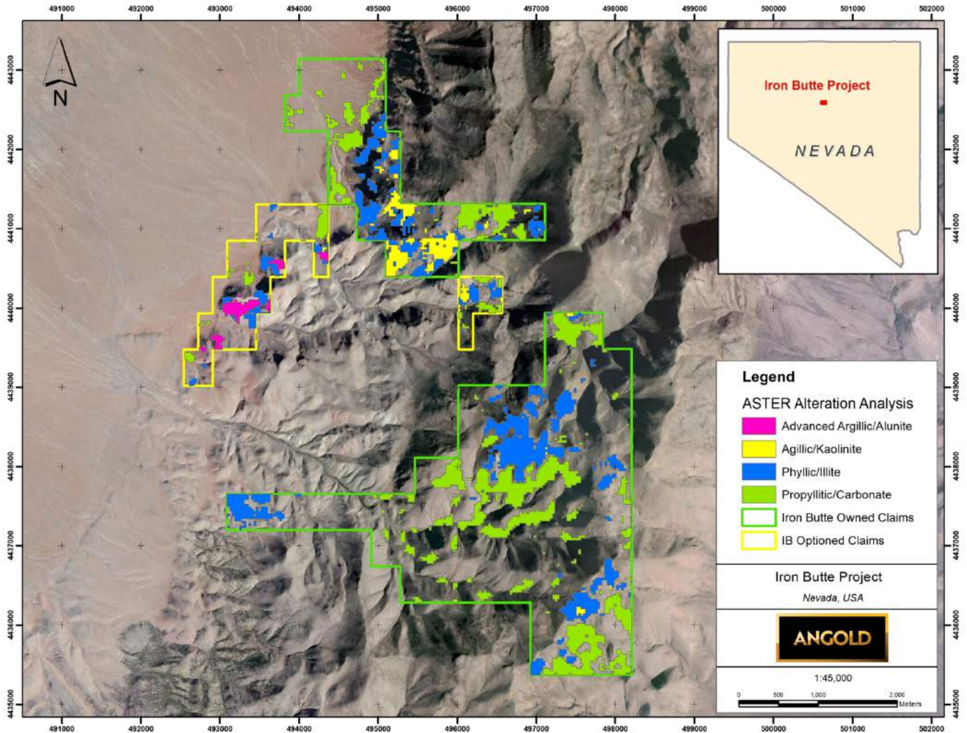
Figure 8. Aster alteration map of Iron Butte properties area.
