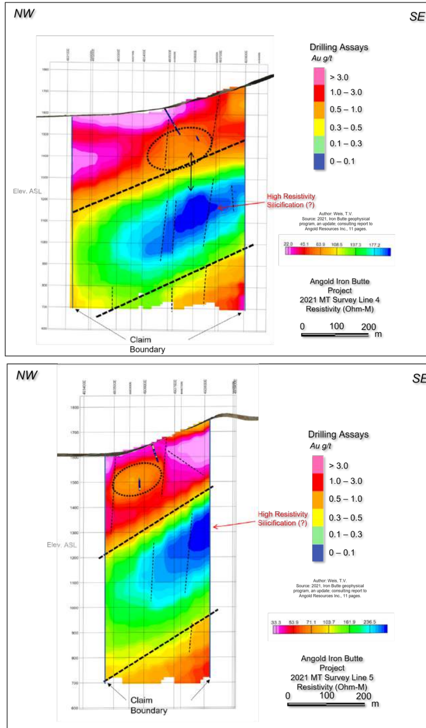
Figure 14. Cross-sections of MT (magnetotelluric) survey results on lines 4 and 5. Heavy dashed black lines interpreted as west-dipping thrust faults; the upper line is the interpreted Golconda thrust fault. Low resistivity (red, pink colors) interpreted as Havallah sequence siltstones in upper plate to the Golconda thrust. Drill holes superimposed on section show that most holes remained in the upper plate. High resistivity (blue, green) interpreted as strong-moderate silicification in lower plate to Golconda thrust. Vertical dashed lines interpreted as normal faults, some of which broke through Golconda thrust and carried altering, moderate-weak silicification (yellow, orange; dotted ellipses) and mineralizing fluids into upper plate
