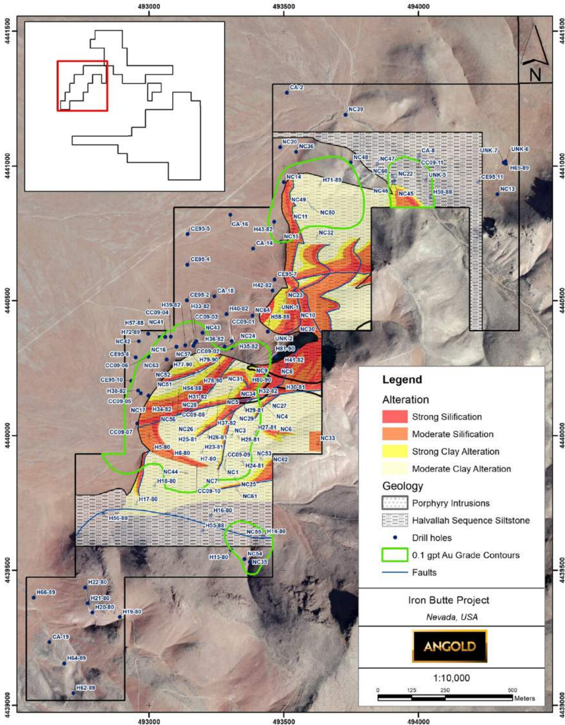
Figure 7. Geologic map of center of optioned Iron Butte property showing normal fault-controlled silica-rich alteration (red) and extensive clay alteration (yellow) of Havallah sequence siltstone (dashed lines) and porphyry intrusion (x pattern) host rocks. Also shown, reverse circulation drill holes drilled by previous companies (1980-2009) and outlines of >0.1 g/t Au based on drill results.
