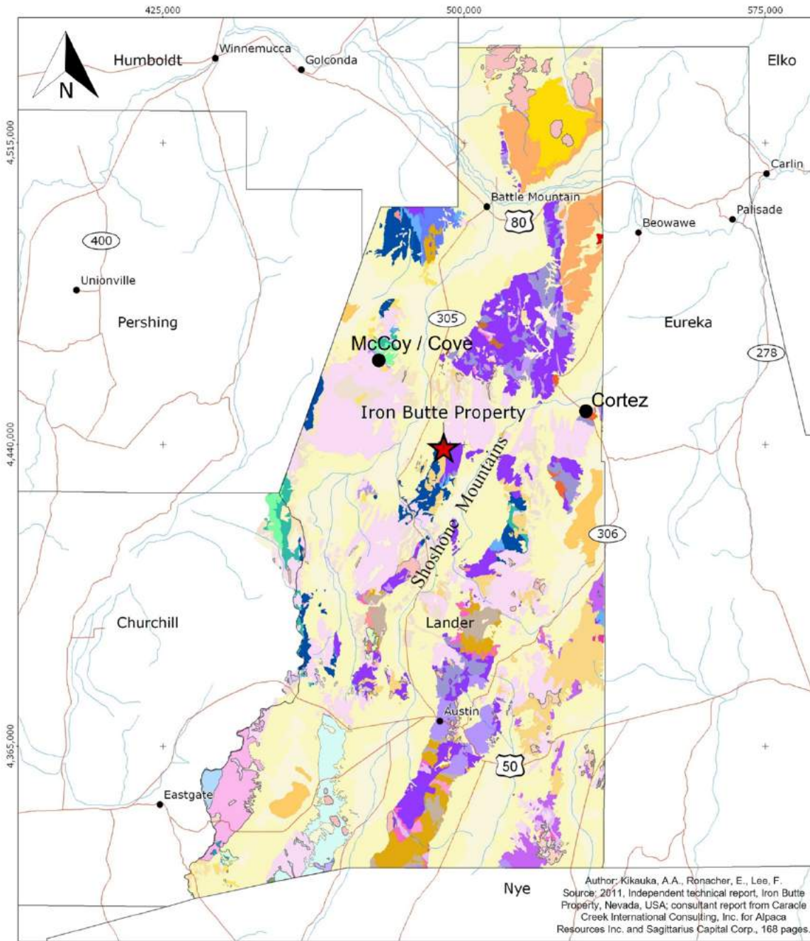
Figure 1. Location of Iron Butte properties on geologic map of Lander County, Nevada. Also shown, McCoy/Cove and Cortez mining districts.
