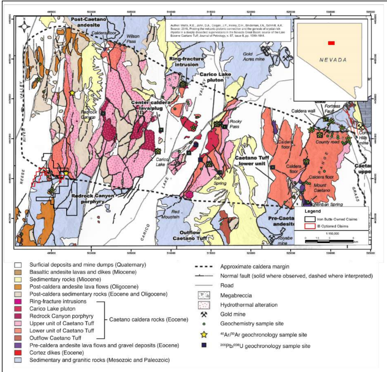
Figure 5. Geologic map of Caetano caldera showing Cortez district gold deposits adjacent to northeast margin and Iron Butte properties adjacent to southwest margin.
