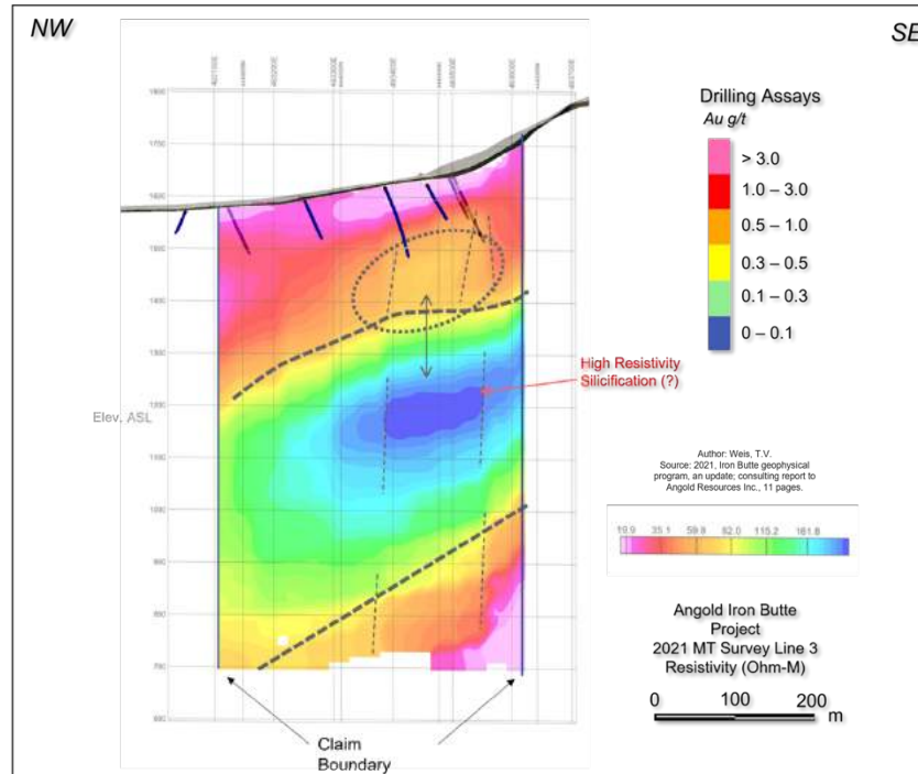
Figure 13. Cross-sections of MT (magnetotelluric) survey results on lines 2 and 3. Heavy dashed black lines interpreted as west-dipping thrust faults; the upper line is the interpreted Golconda thrust fault. Low resistivity (red, pink colors) interpreted as Havallah sequence siltstones in upper plate to the Golconda thrust. Drill holes superimposed on section show that most holes remained in the upper plate. High resistivity (blue, green) interpreted as strong-moderate silicification in lower plate to Golconda thrust. Vertical dashed lines interpreted as normal faults, some of which broke through Golconda thrust and carried altering, moderate-weak silicification (yellow, orange; dotted ellipses) and mineralizing fluids into upper plate
