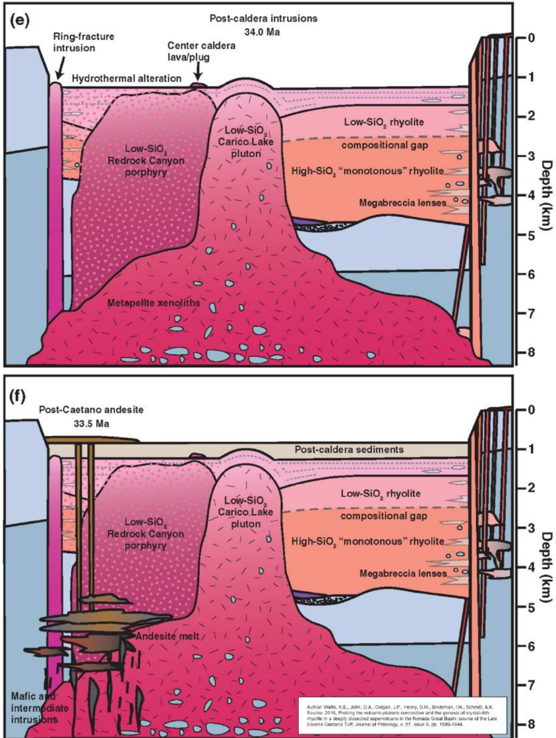
Figure 6. Schematic diagram of evolution of Caetano caldera (34-33.5 Mya). Iron Butte properties located along left margin of caldera adjacent to ring-fracture intrusion, hydrothermal alteration, Redrock Canyon porphyry intrusion, and post Caetano andesite.
