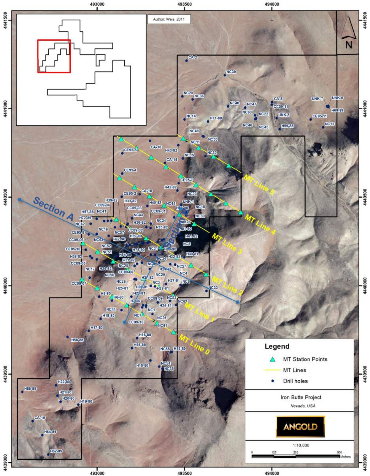
Figure 11. Map of MT (magnetotelluric) survey lines on optioned Iron Butte property.
