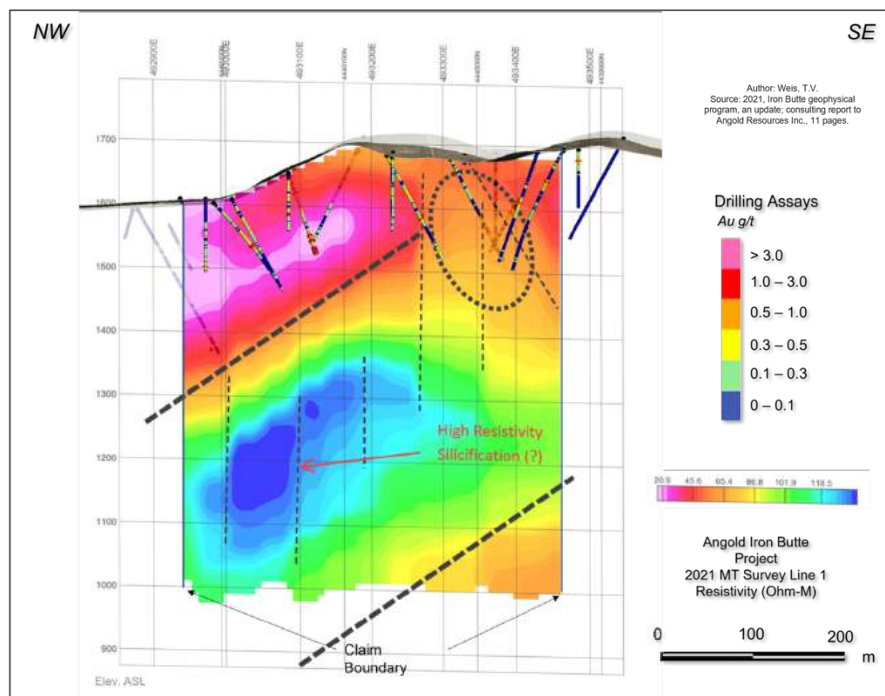
Figure 12. Cross-sections of MT (magnetotelluric) survey results on lines 0 and 1. Heavy dashed black lines interpreted as west-dipping thrust faults; the upper line is the interpreted Golconda thrust fault. Low resistivity (red, pink colors) interpreted as Havallah sequence siltstones in upper plate to the Golconda thrust. Drill holes superimposed on section show that most holes remained in the upper plate. High resistivity (blue, green) interpreted as strong-moderate silicification in lower plate to Golconda thrust. Vertical dashed lines interpreted as normal faults, some of which broke through Golconda thrust and carried altering, moderate-weak silicification (yellow, orange; dotted ellipses) and mineralizing fluids into upper plate
