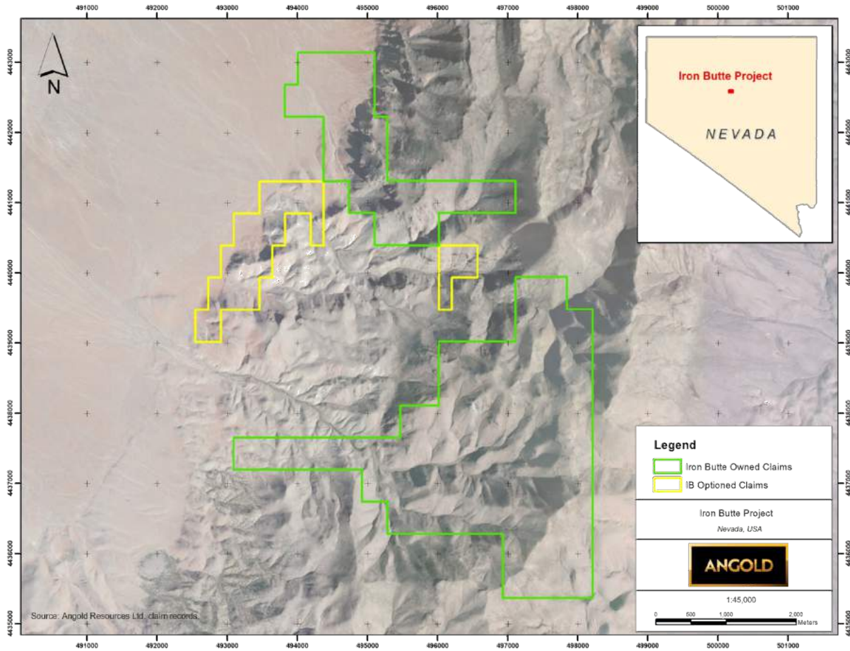
Figure 2. Location of Iron Butte properties on satellite image.
