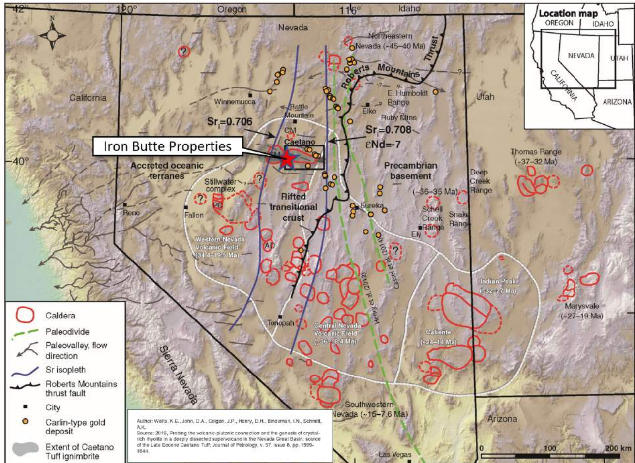
Figure 4. Location of Tertiary volcanic calderas, Nevada and Utah. Caetano caldera with Cortez gold deposits shown along northeast caldera margin.
